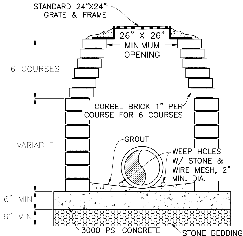
SECTION
